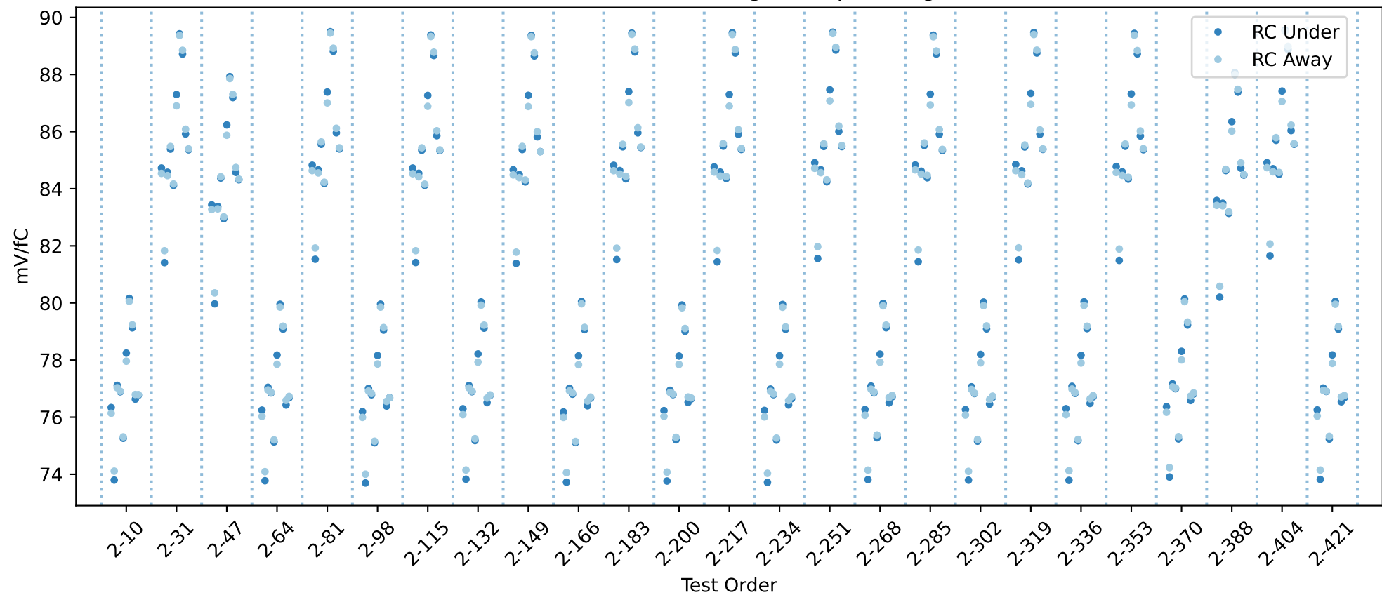
20USBHX2005521 RC gain chip averages
