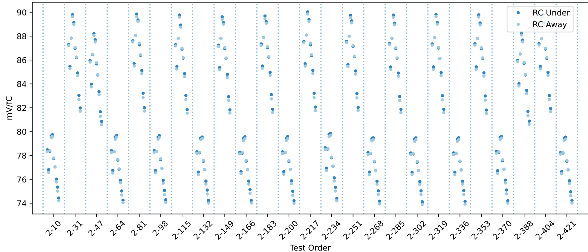
20USBHX2005522 RC gain chip averages
