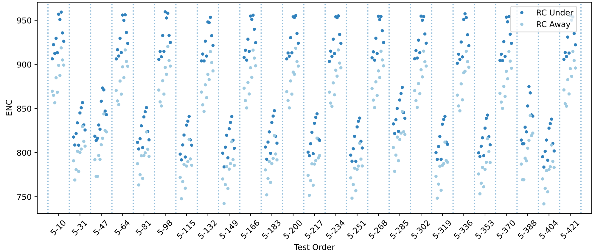
20USBHX2005525 RC innse chip averages
