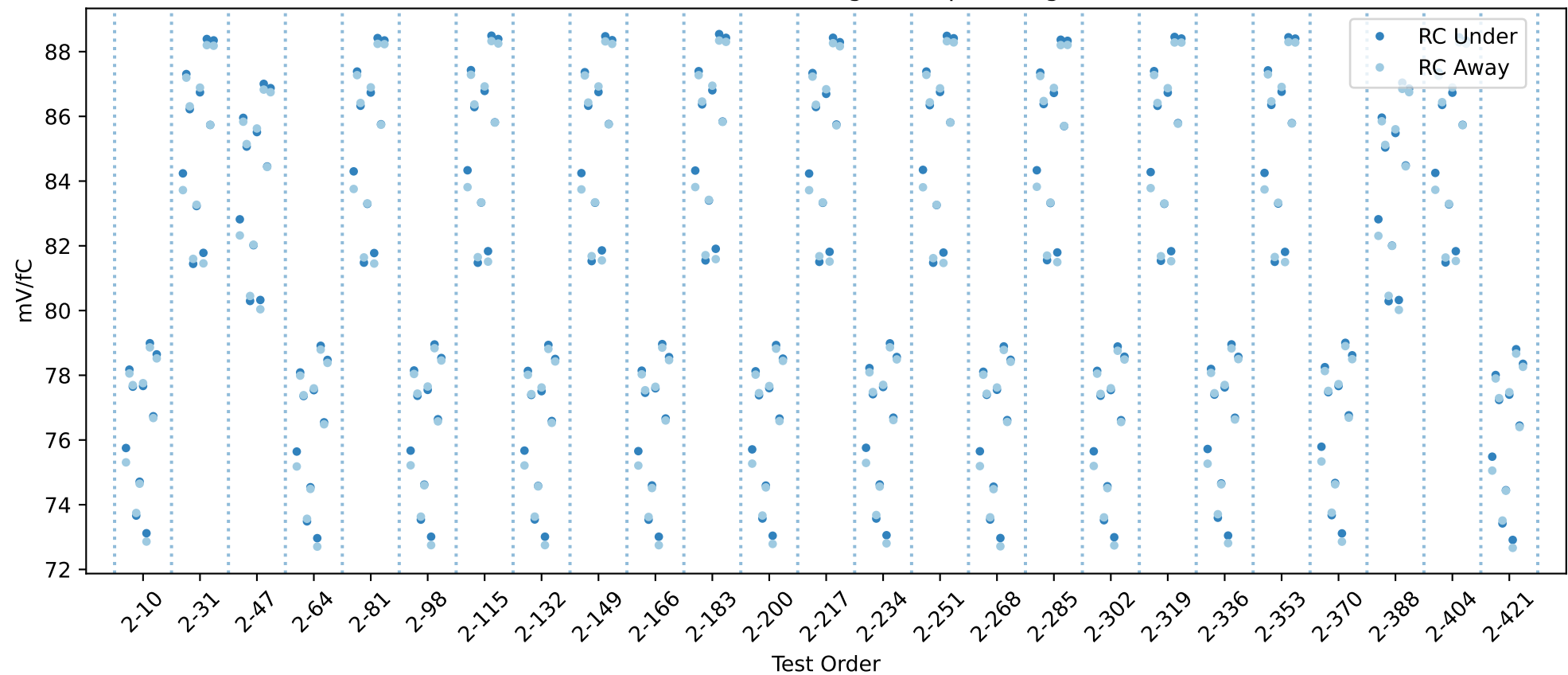
20USBHX2005516 RC gain chip averages
