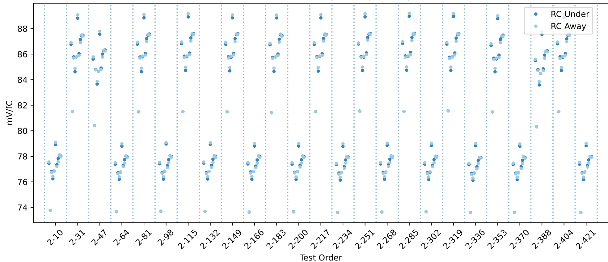
20USBHX2005564 RC gain chip averages
