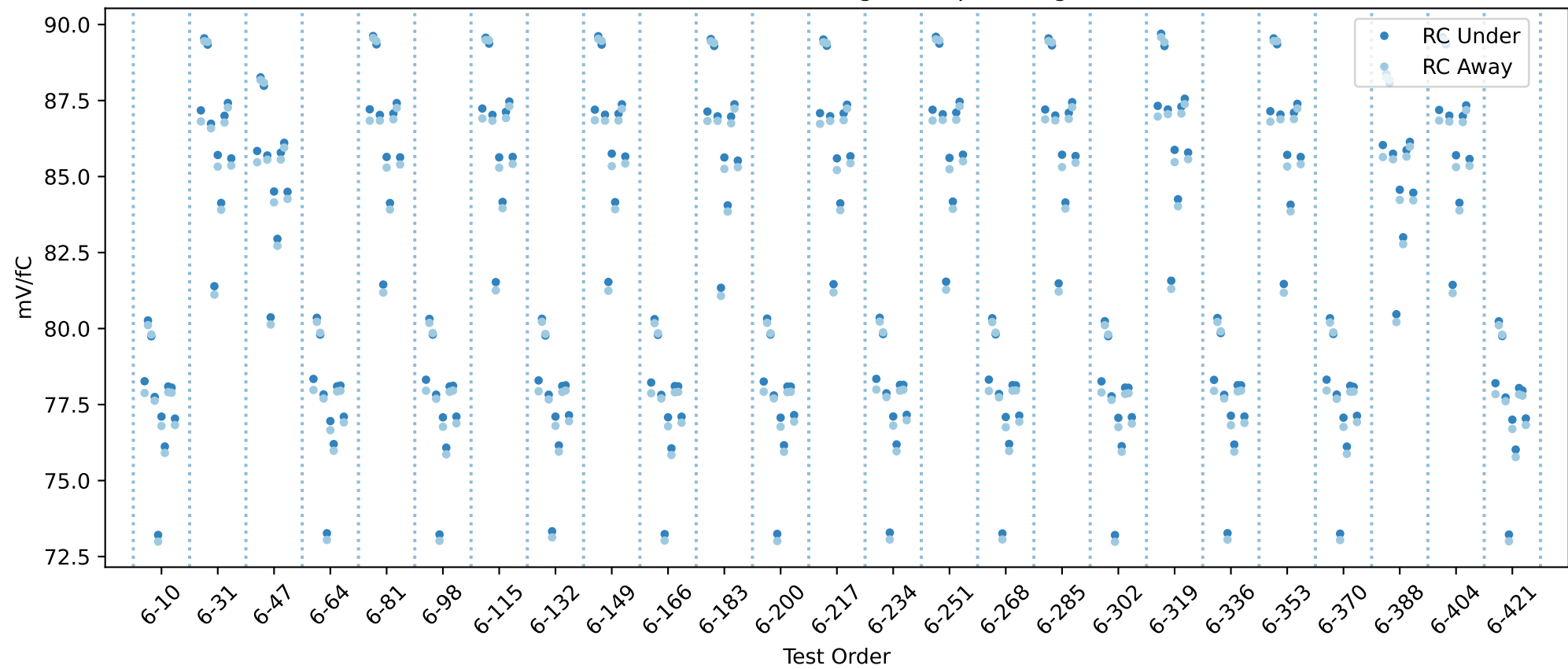
20USBHX2005289 RC gain chip averages
