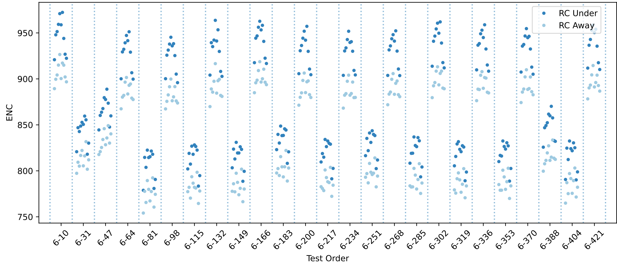
20USBHX2005289 RC innse chip averages
