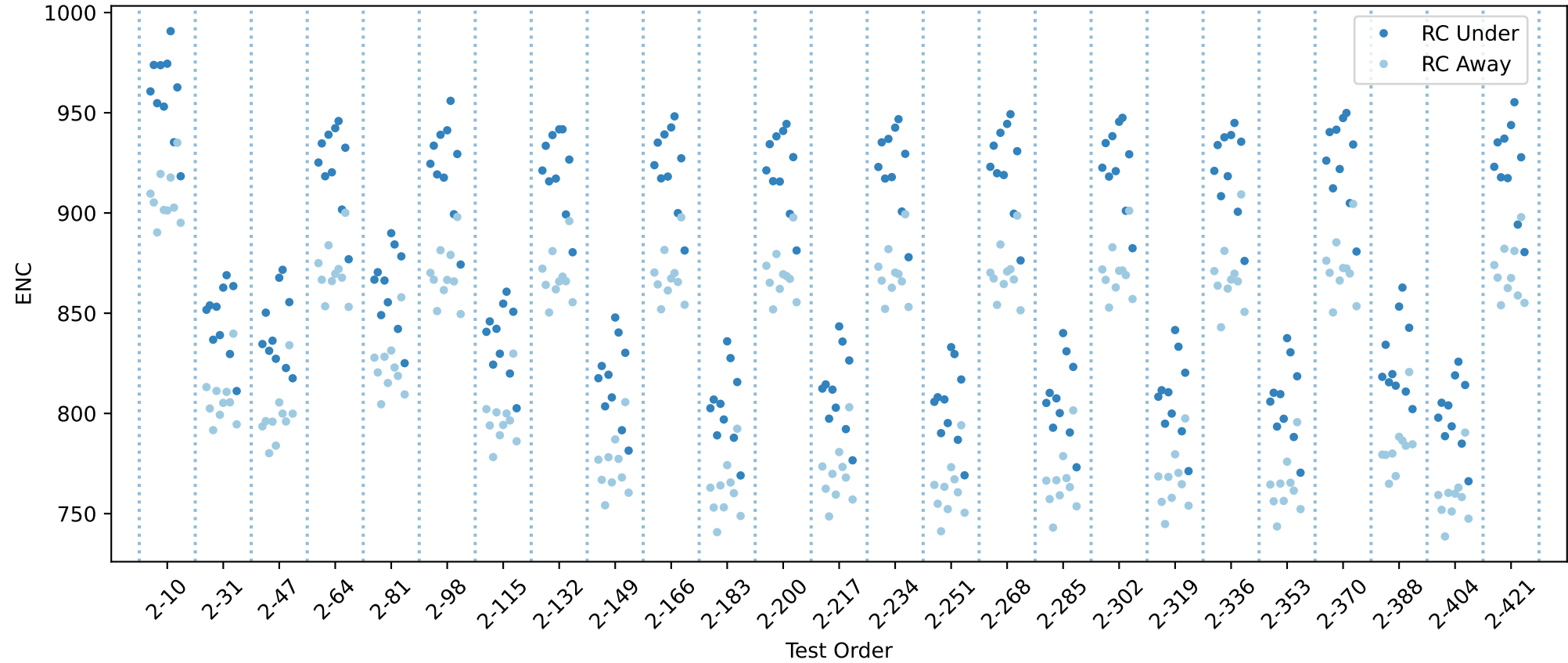
20USBHX2005290 RC innse chip averages
