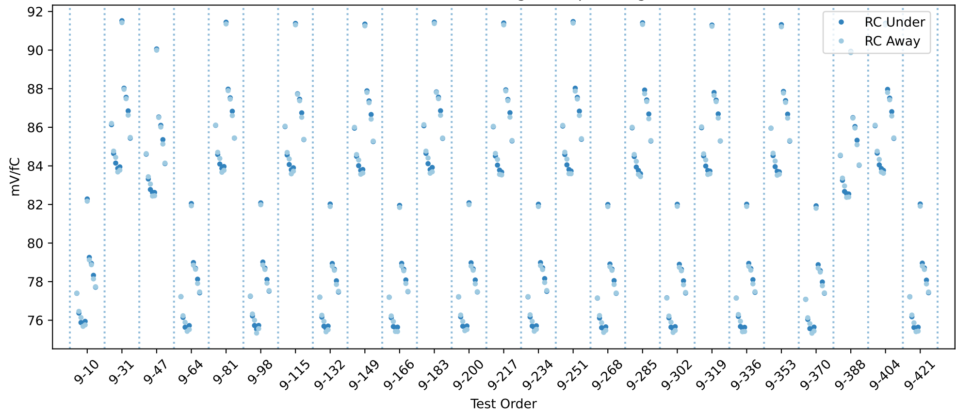
20USBHX2005242 RC gain chip averages
