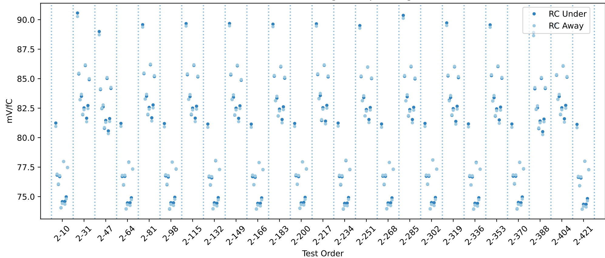
20USBHX2005281 RC gain chip averages
