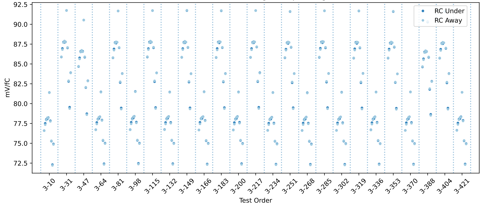
20USBHX2004873 RC gain chip averages
