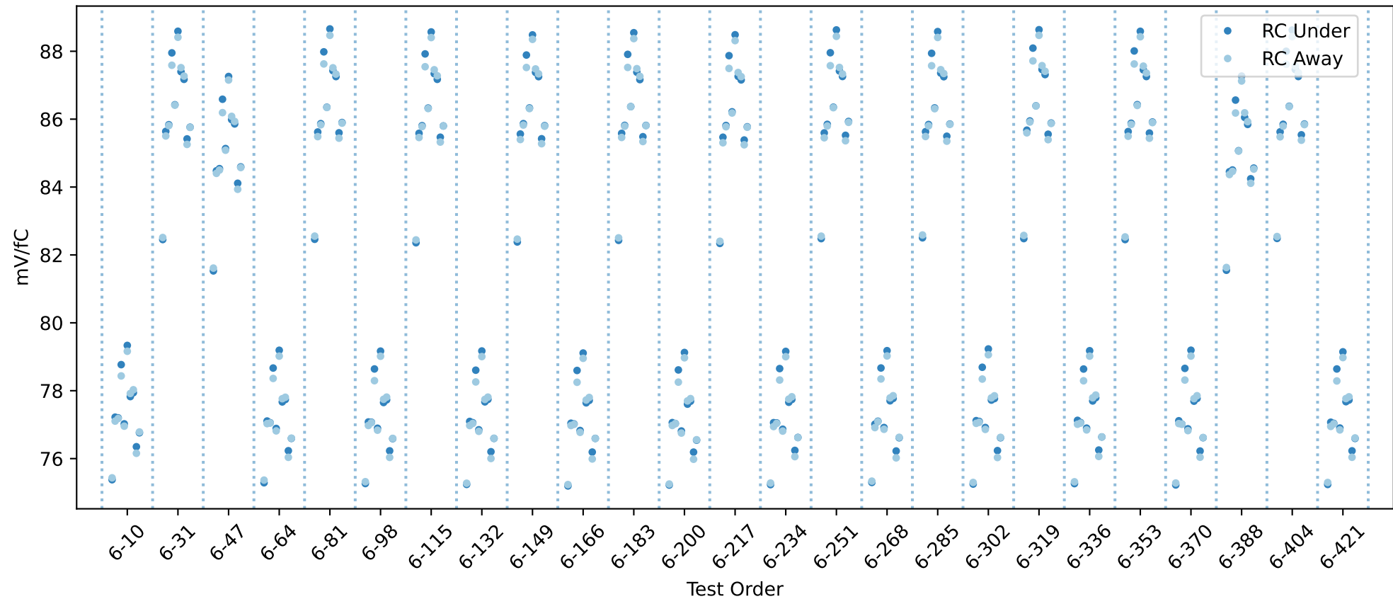
20USBHX2004849 RC gain chip averages
