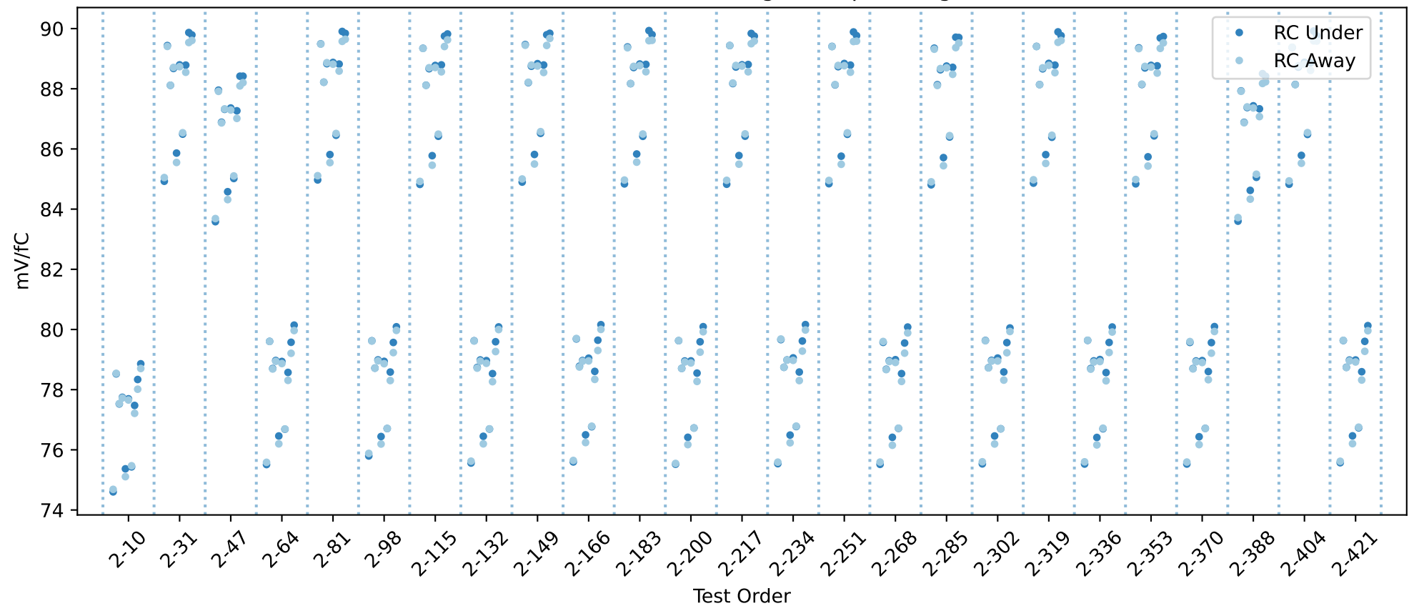
20USBHX2005244 RC gain chip averages
