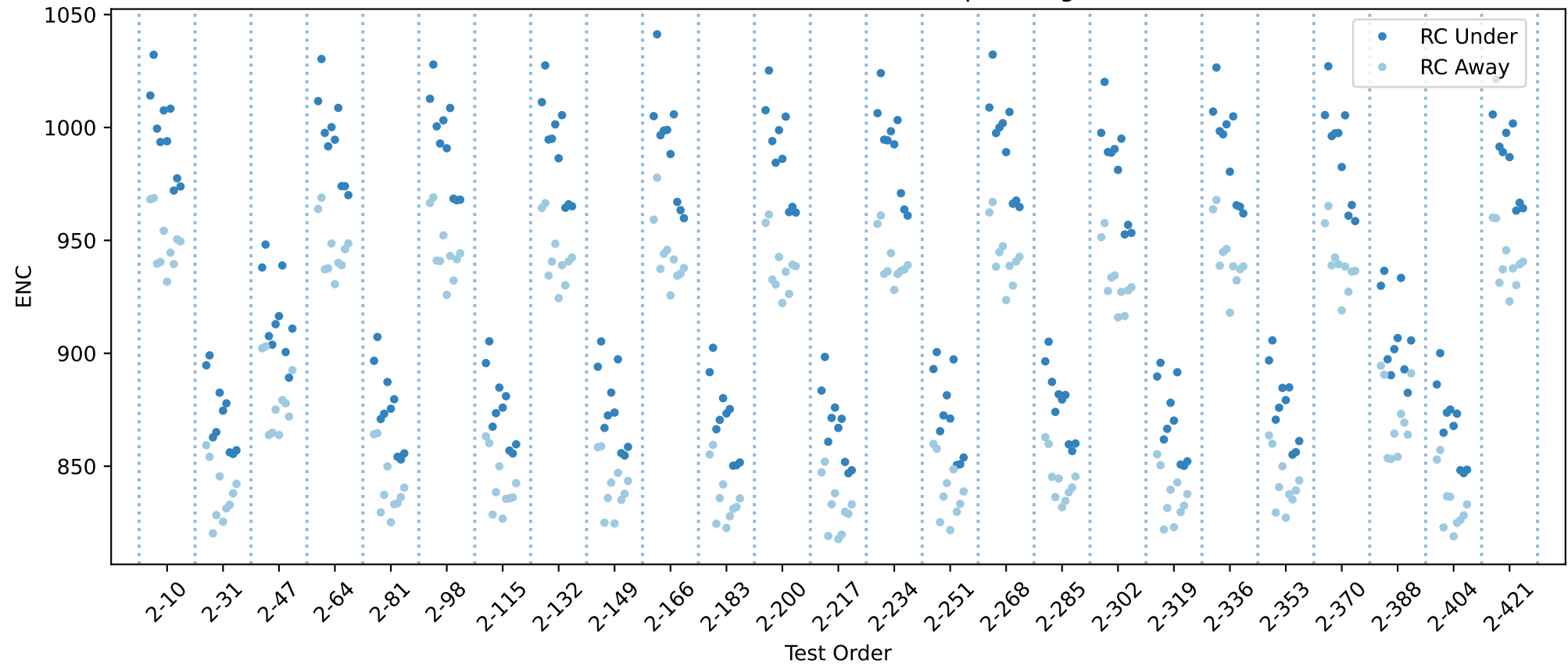
20USBHX2005245RC innse chip averages
