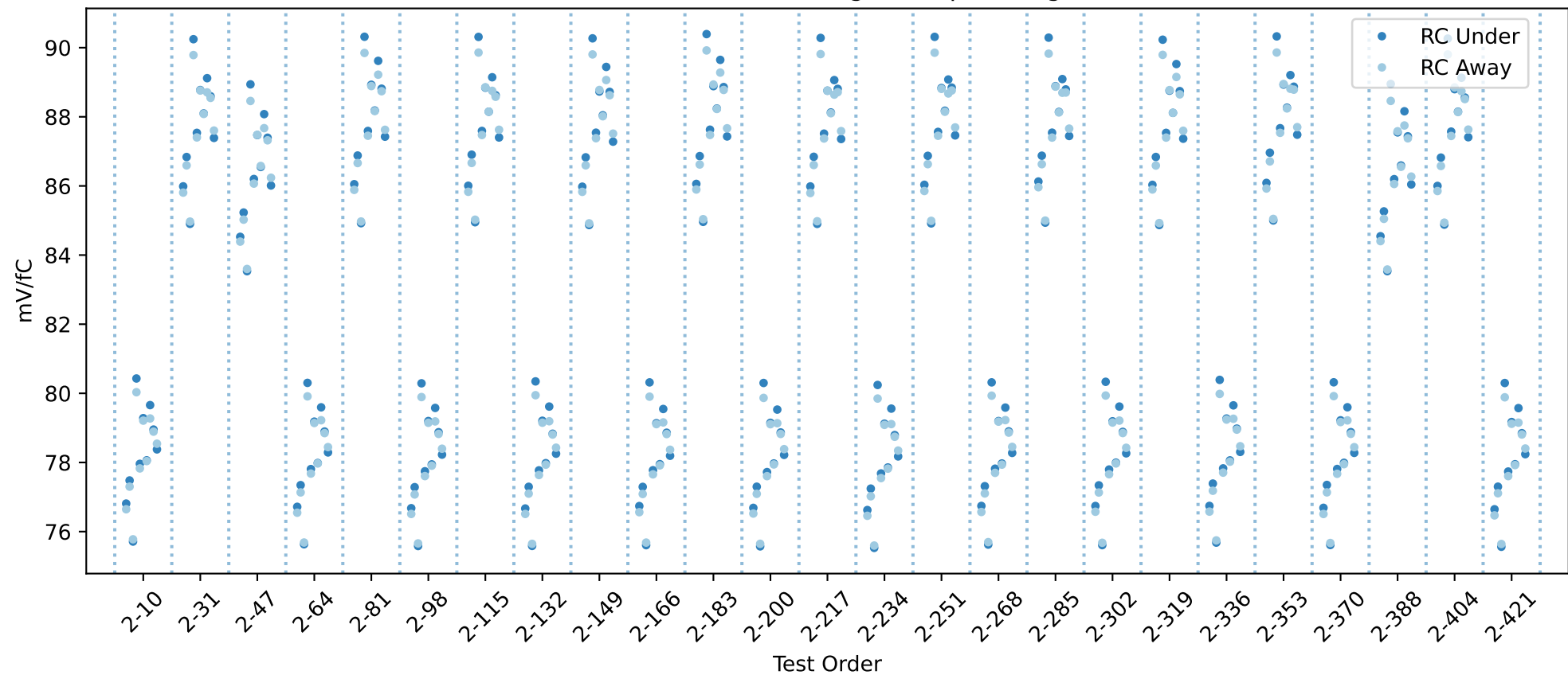
20USBHX2005246 RC gain chip averages
