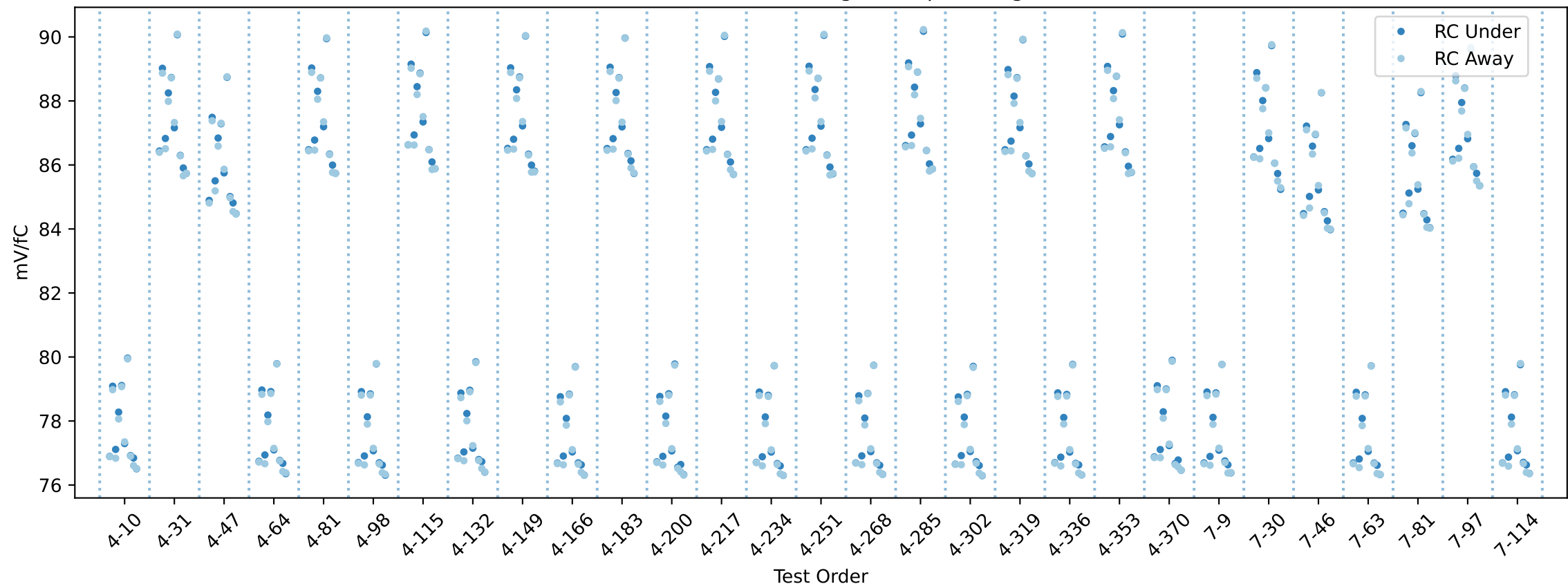
20USBHX2004999 RC gain chip averages
