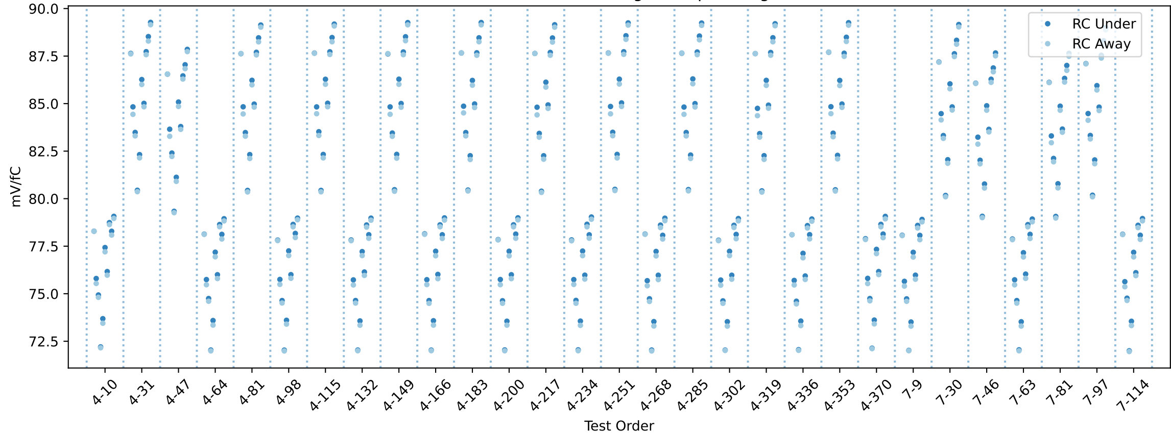
20USBHX2005000 RC gain chip averages
