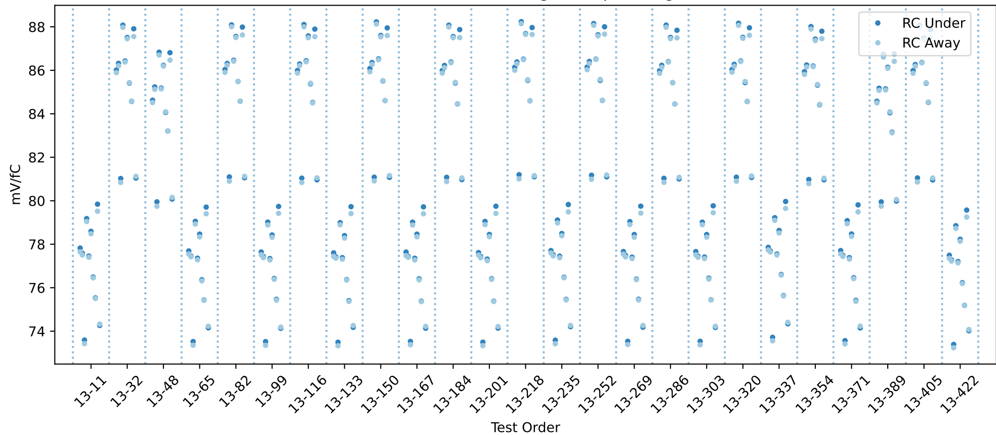
20USBHX2005551 RC gain chip averages
