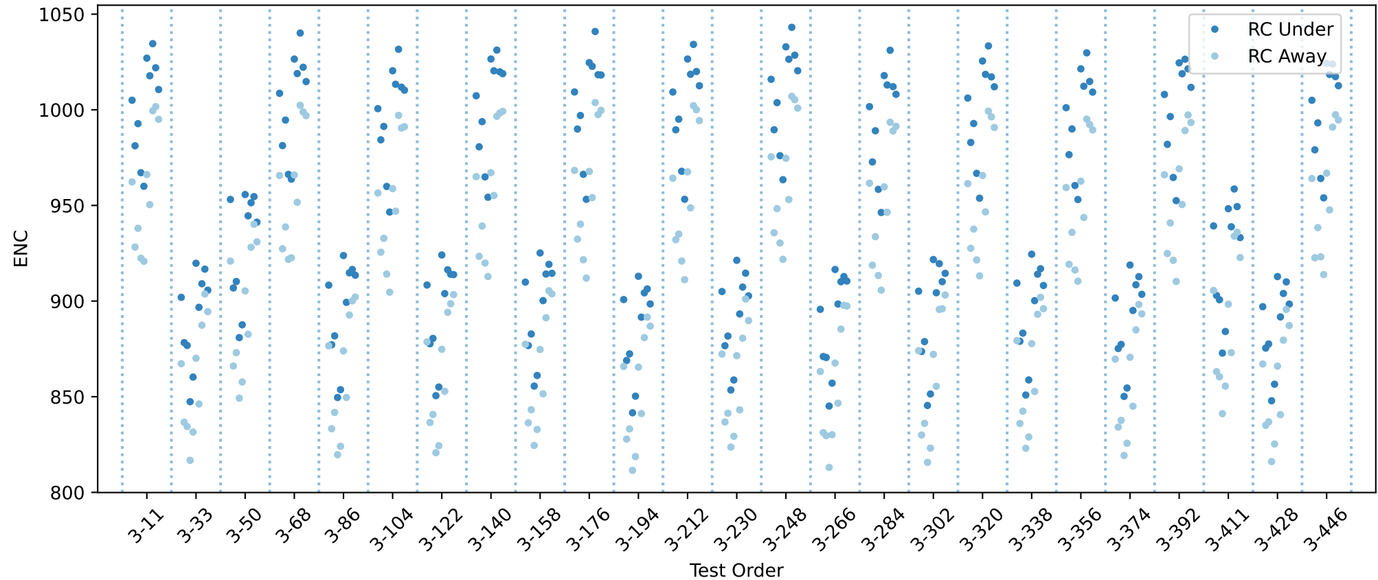
20USBHX2005556 RC innse chip averages
