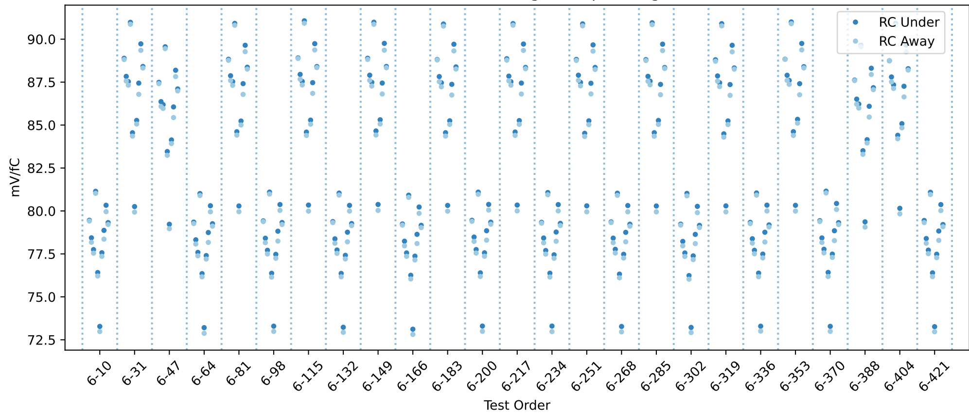
20USBHX2005559 RC gain chip averages
