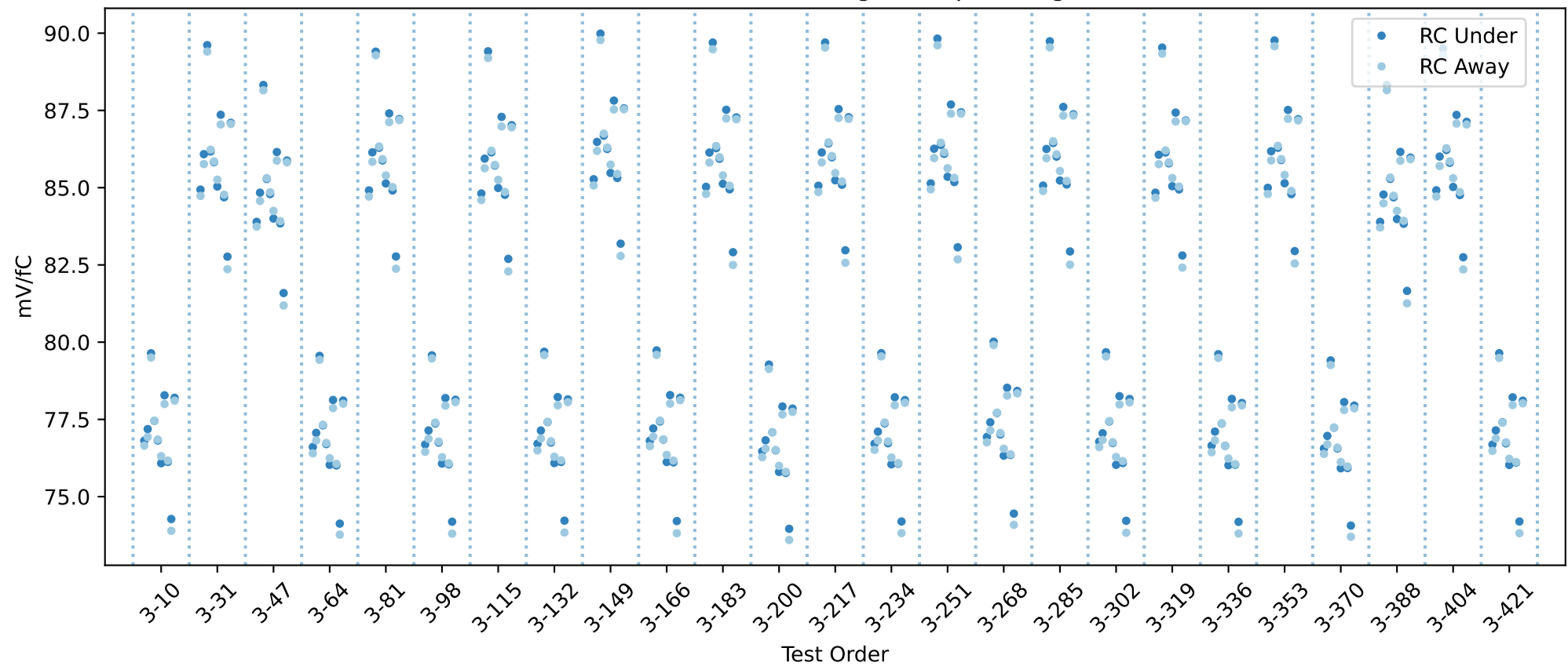
20USBHX2005545 RC gain chip averages
