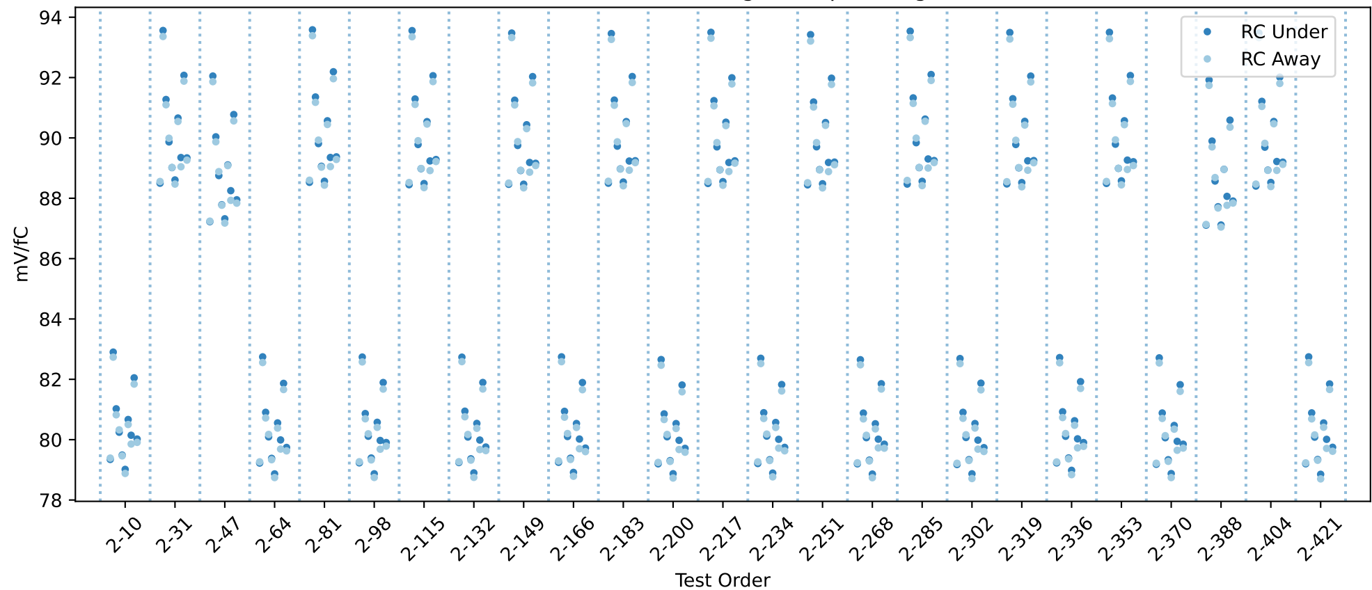
20USBHX2005960 RC gain chip averages
