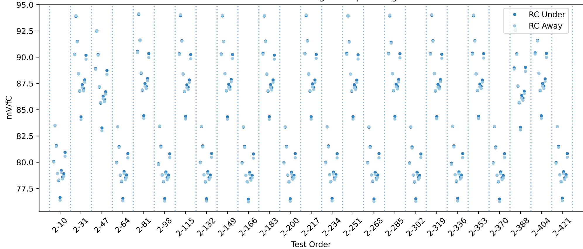
20USBHX2005963 RC gain chip averages
