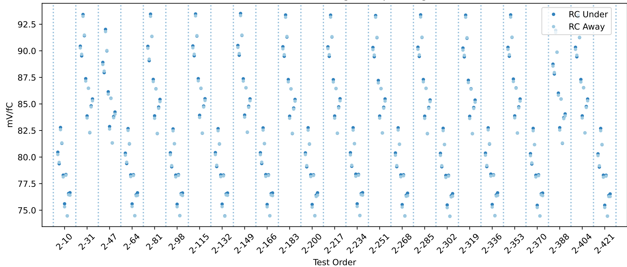
20USBHX2005959 RC gain chip averages
