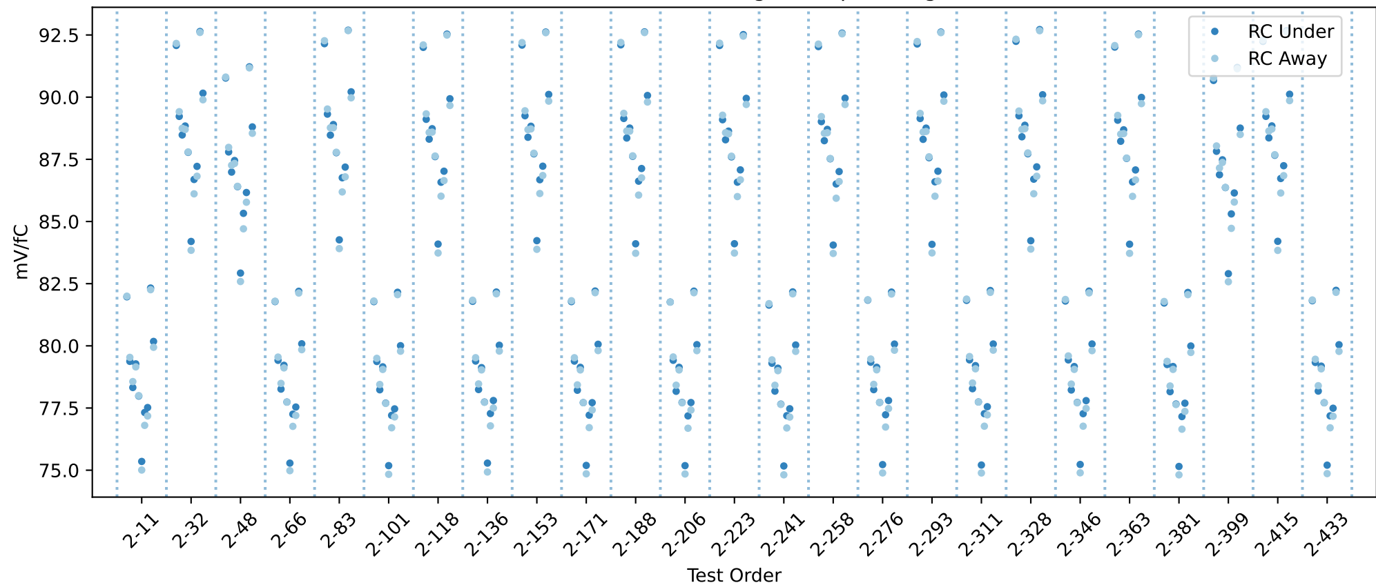
20USBHX2005965 RC gain chip averages
