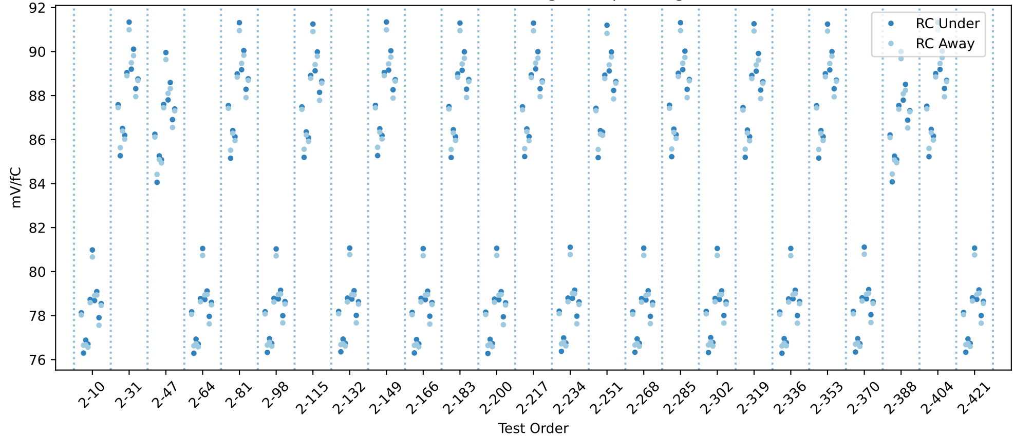
20USBHX2005969 RC gain chip averages
