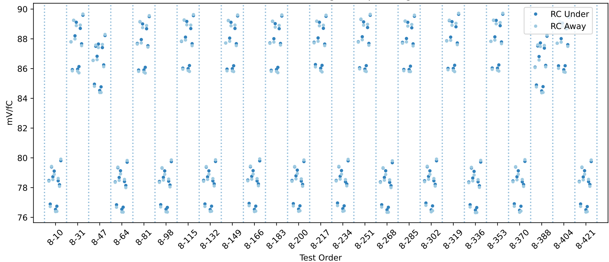
20USBHX2005987 RC gain chip averages
