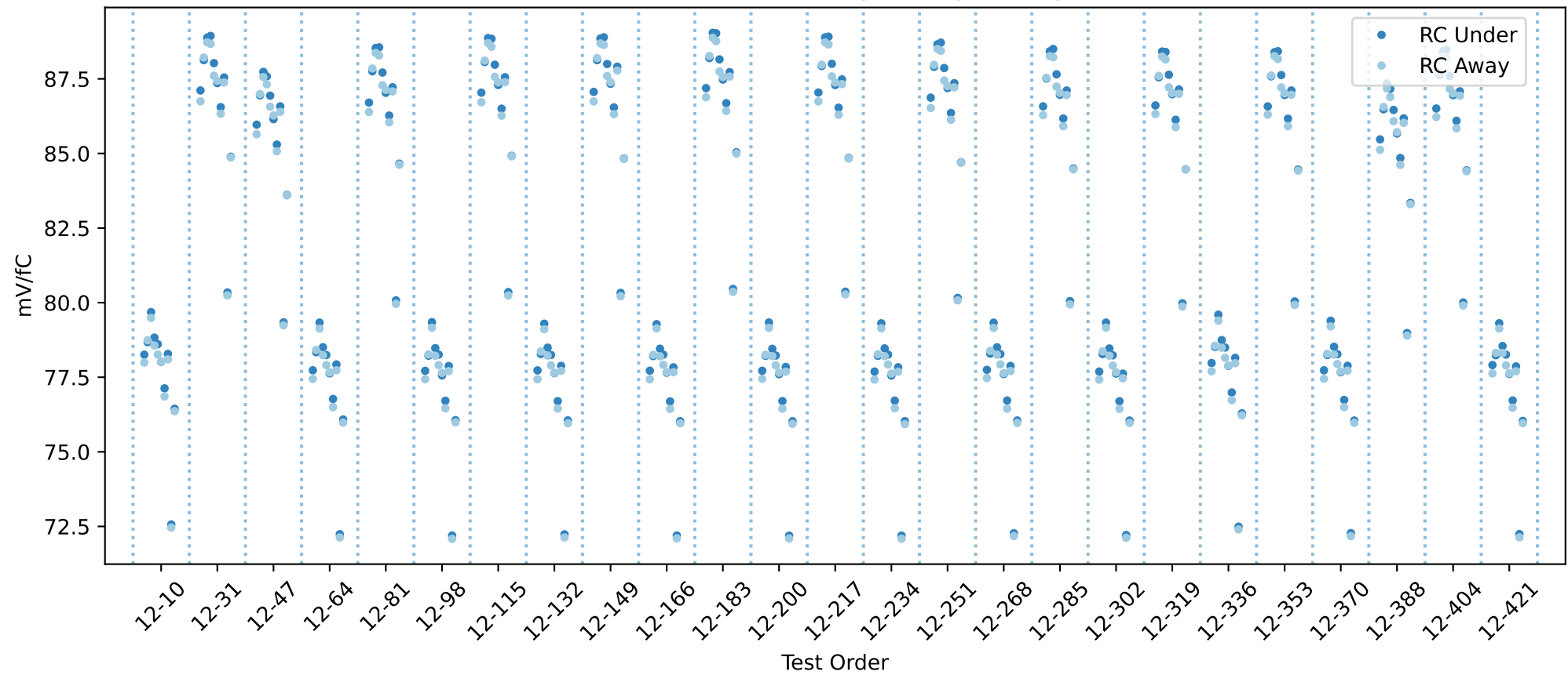
20USBHX2005988 RC gain chip averages
