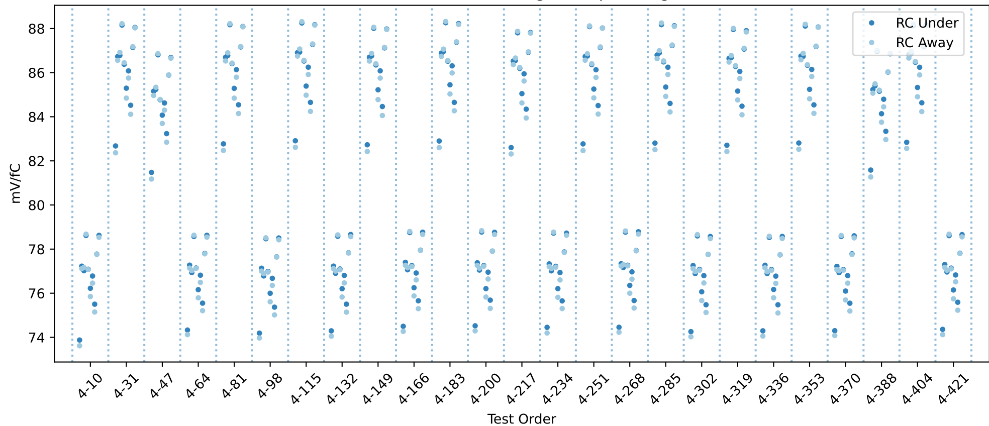
20USBHX2005991 RC gain chip averages
