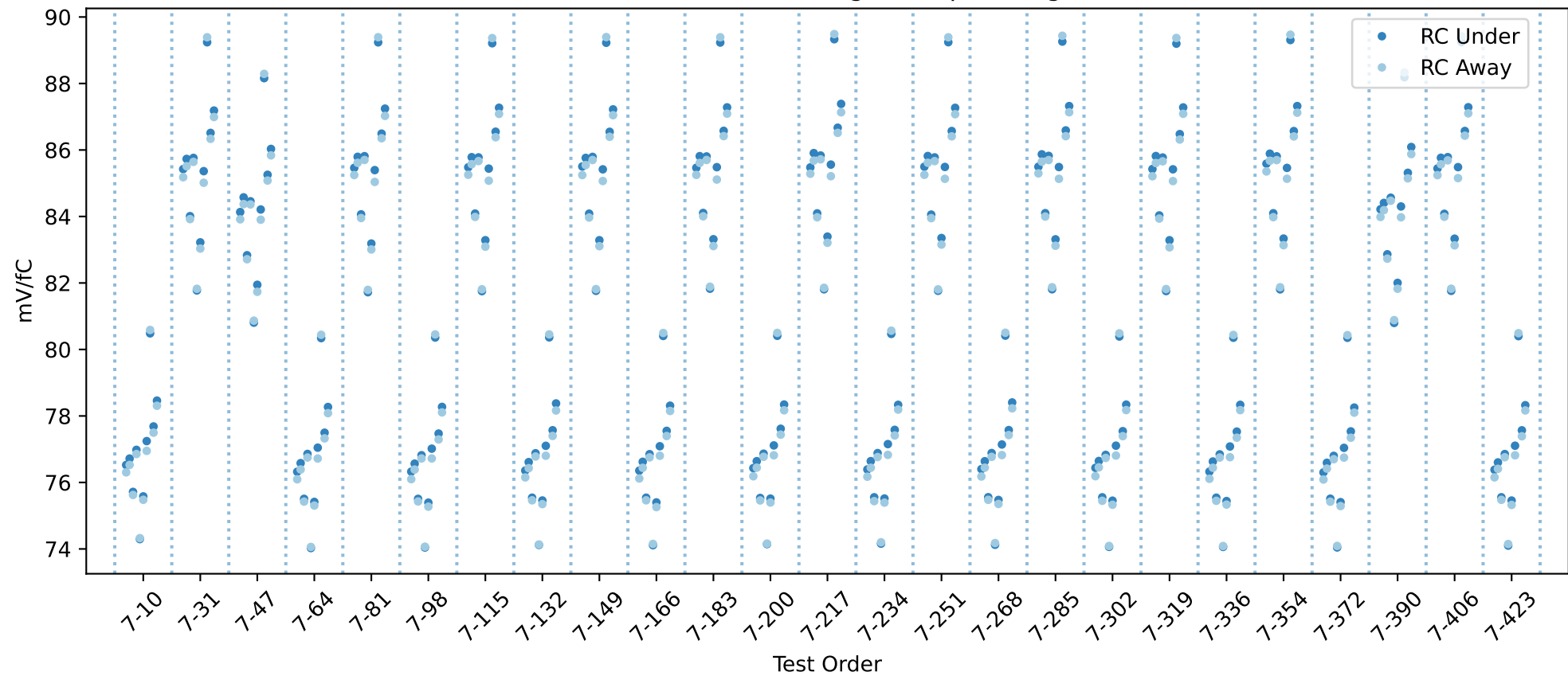
20USBHX2005973 RC gain chip averages
