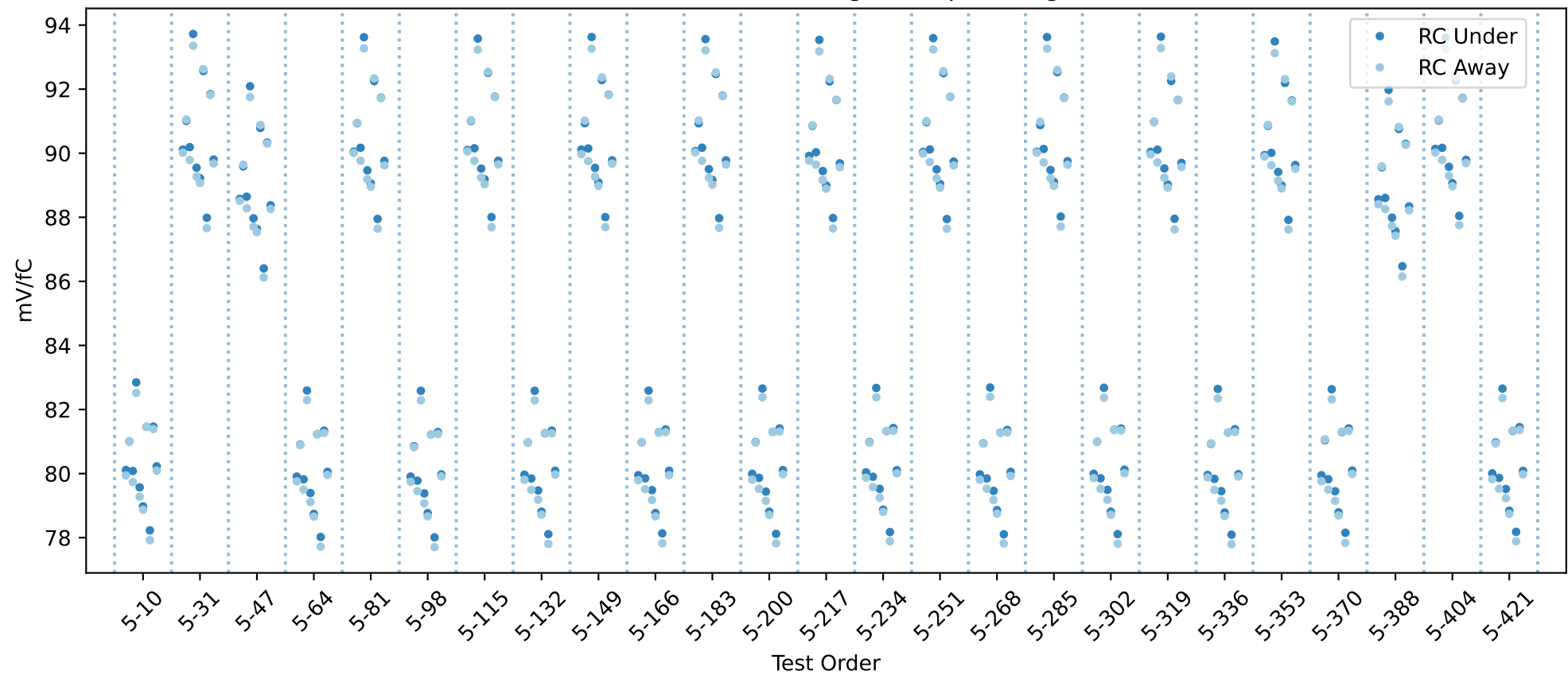
20USBHX2005954 RC gain chip averages
