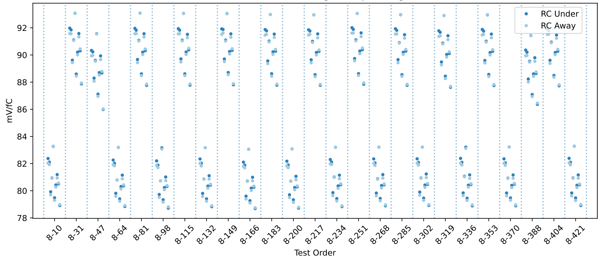
20USBHX2005951 RC gain chip averages
