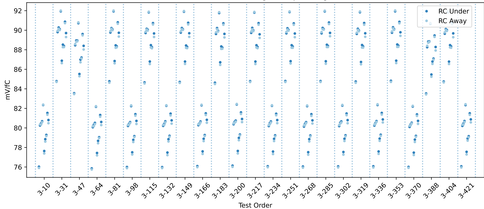
20USBHX2005985 RC gain chip averages
