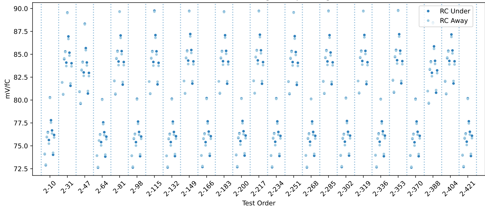
20USBHX2005567 RC gain chip averages
