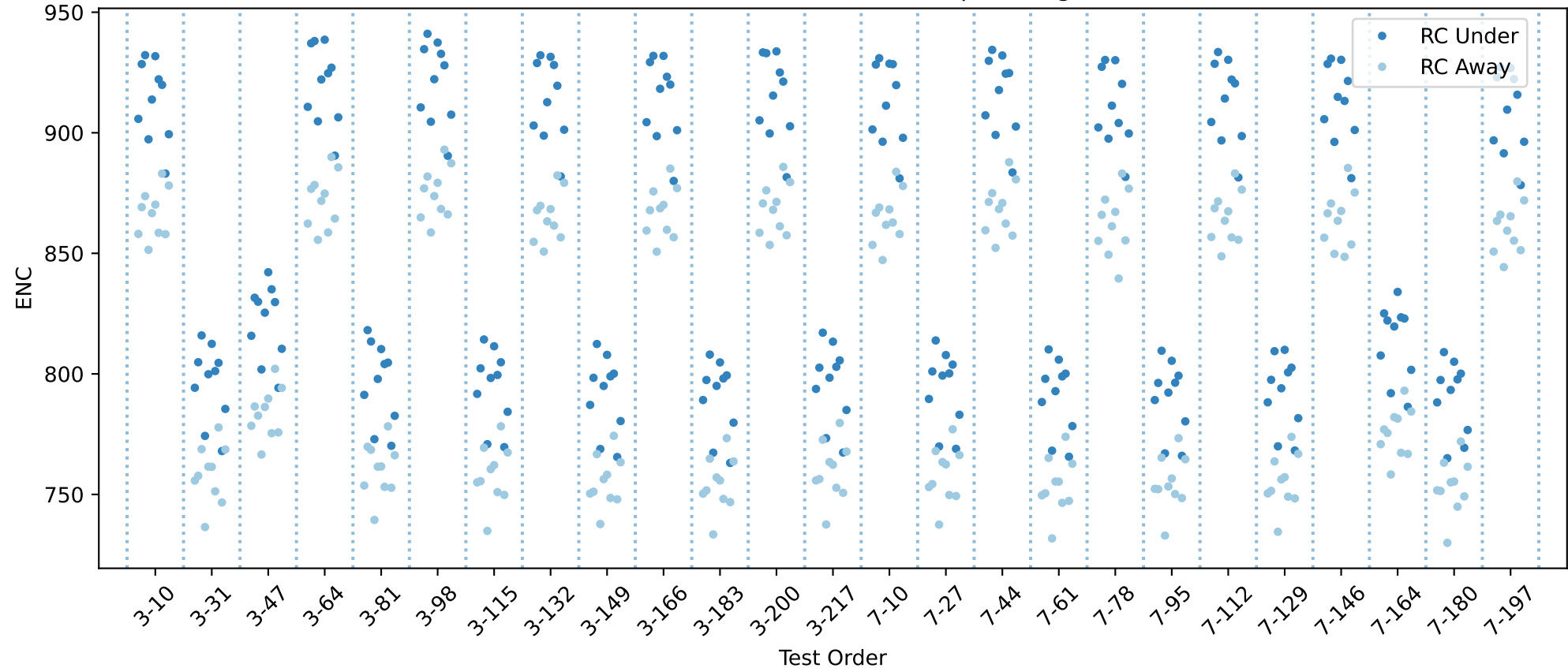
20USBHX2006289 RC innse chip averages
