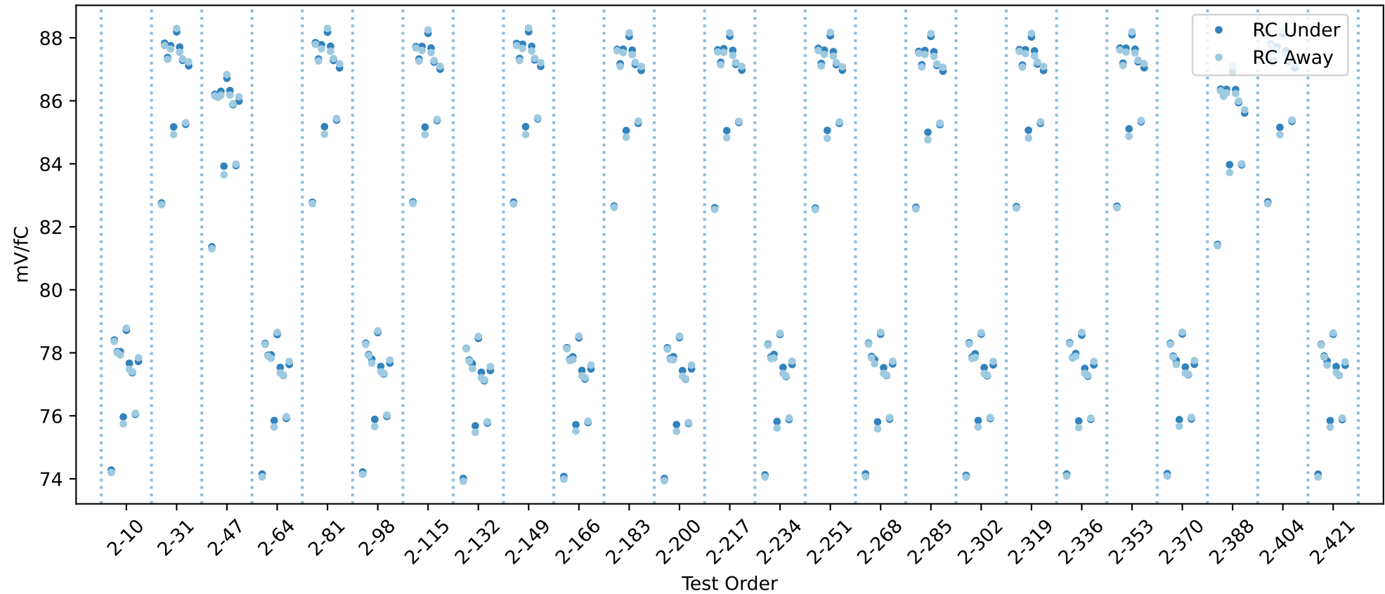
20USBHX2006296 RC gain chip averages
