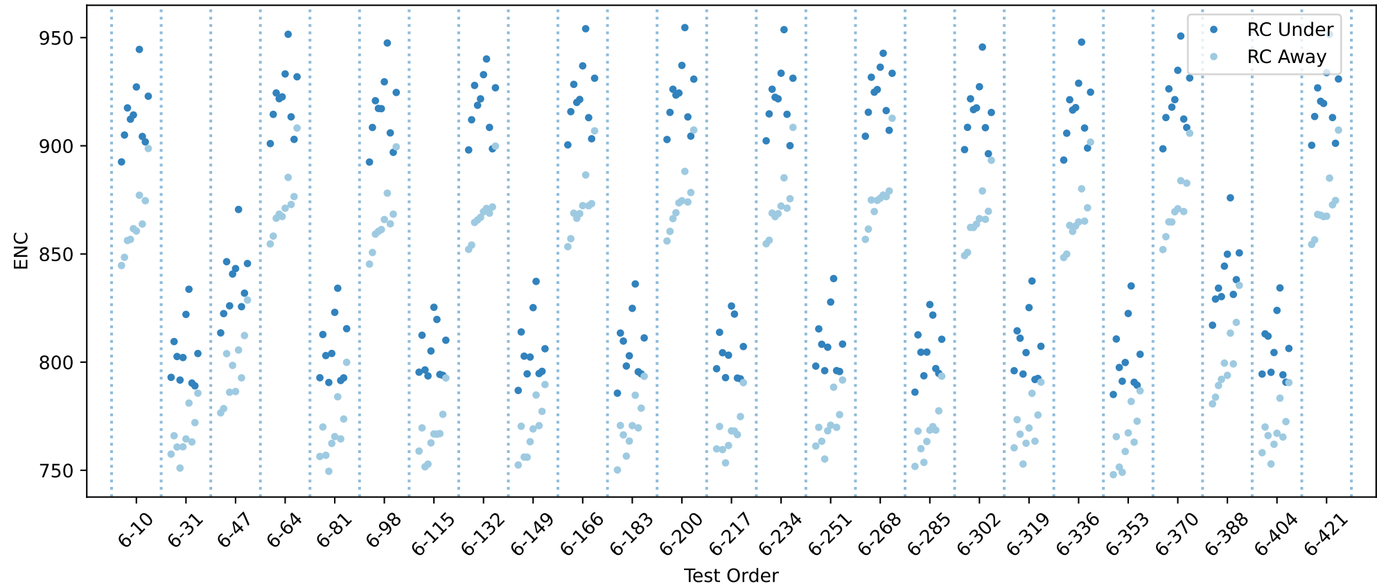
20USBHX2006796 RC innse chip averages
