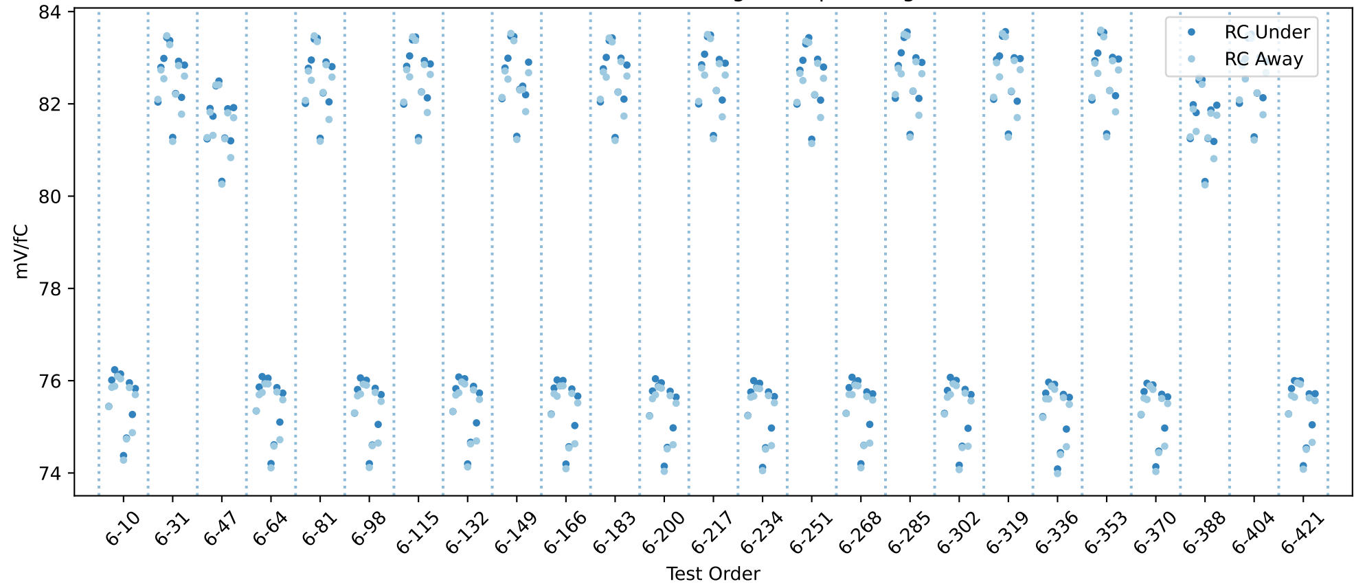
20USBHX2006801 RC gain chip averages
