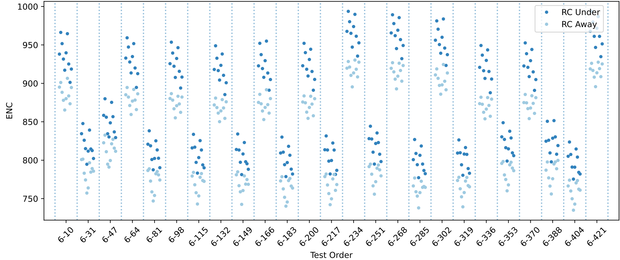
20USBHX2006799 RC innse chip averages
