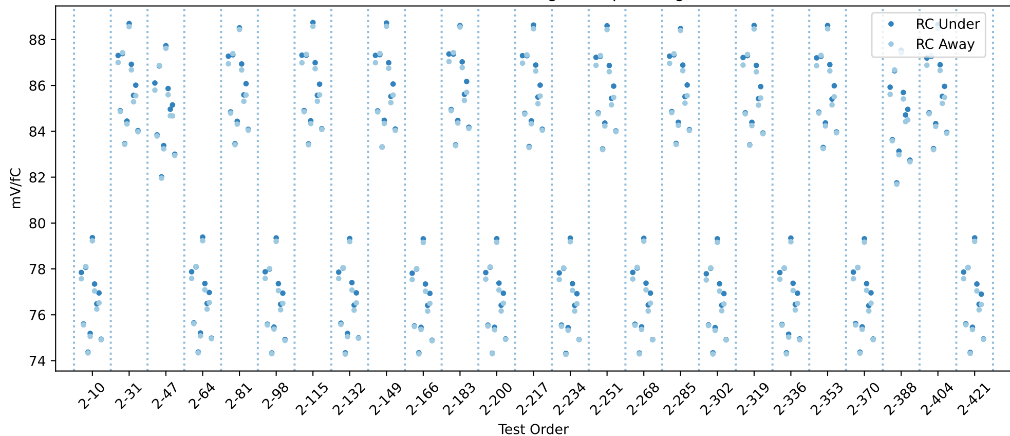
20USBHX2006797 RC gain chip averages
