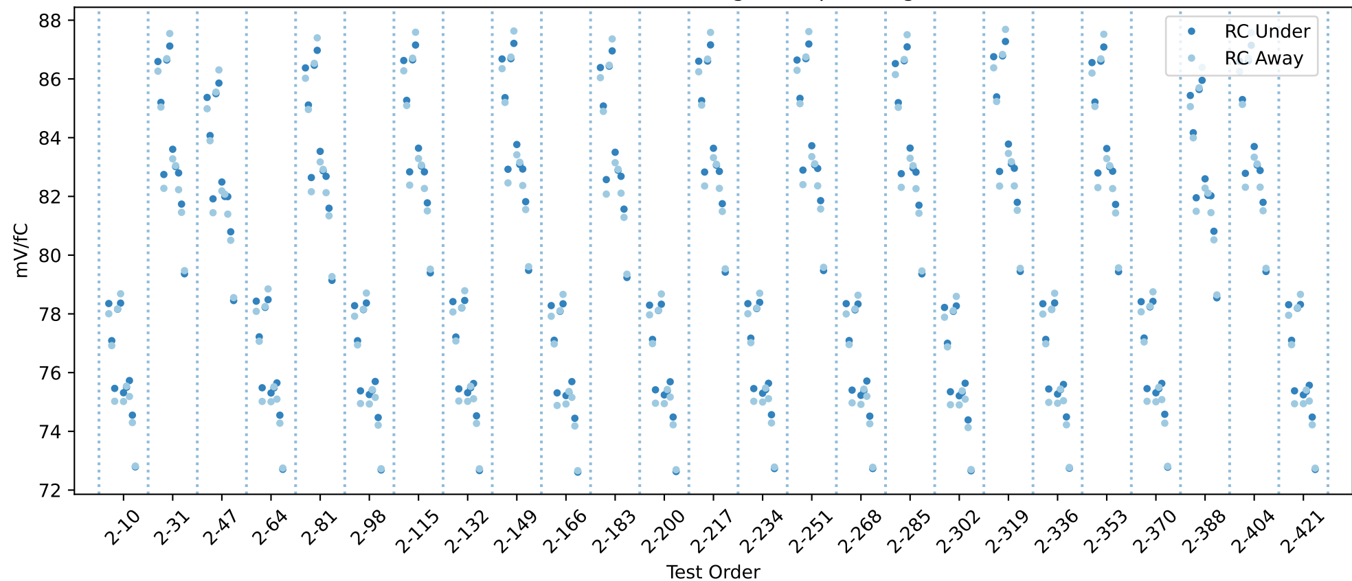
20USBHX2006804 RC gain chip averages
