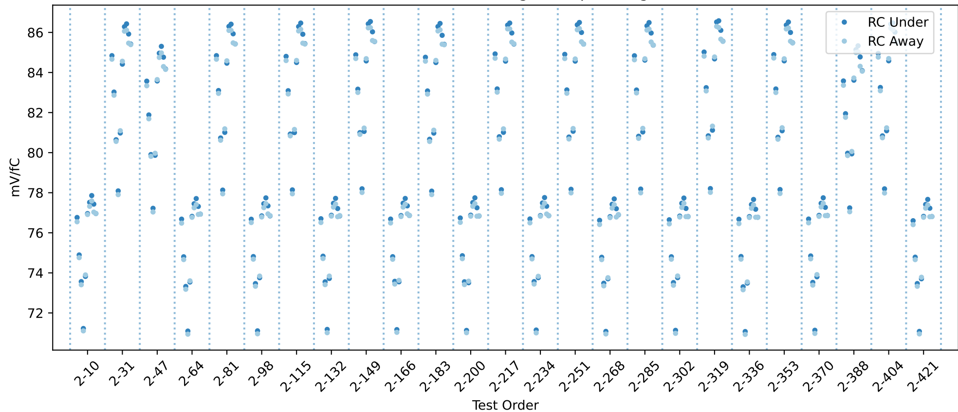
20USBHX2006805 RC gain chip averages
