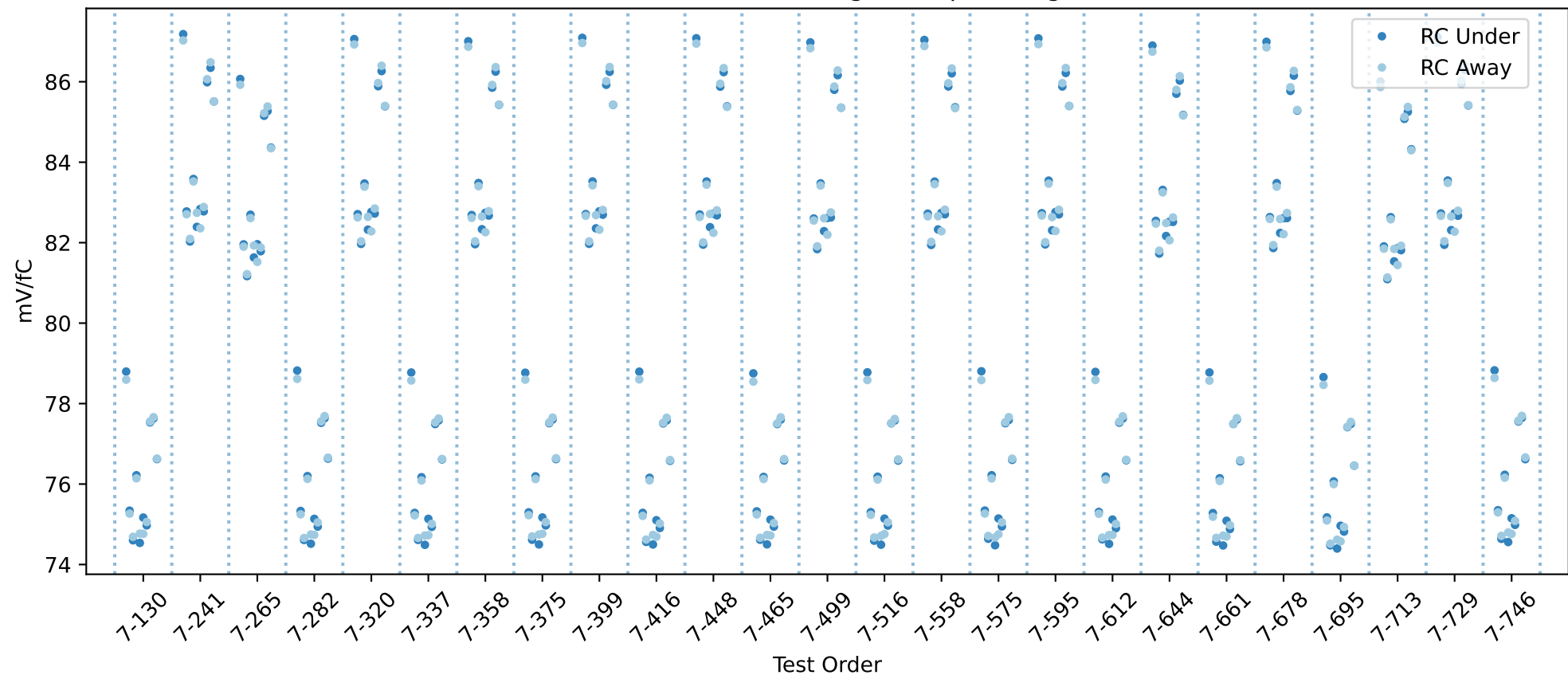
20USBHX2007812 RC gain chip averages
