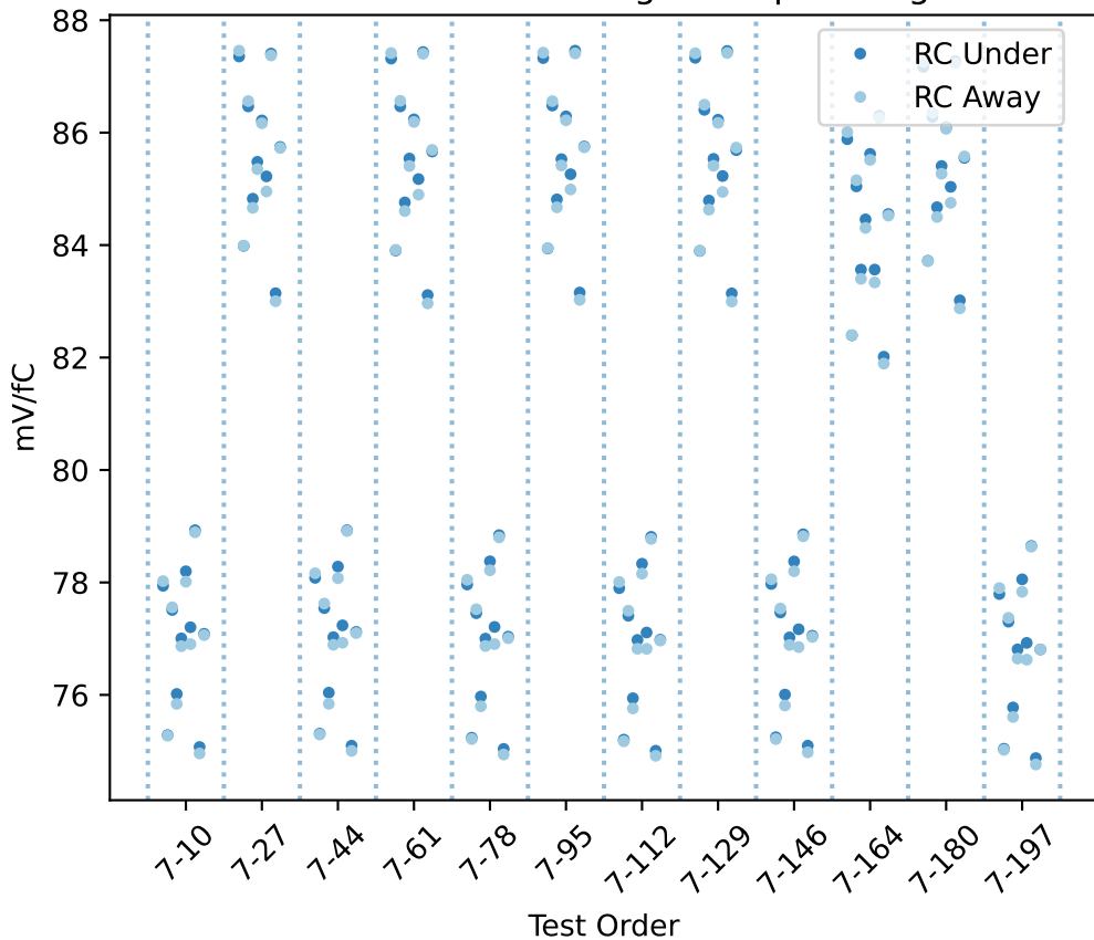
20USBHX2007924 RC gain chip averages
