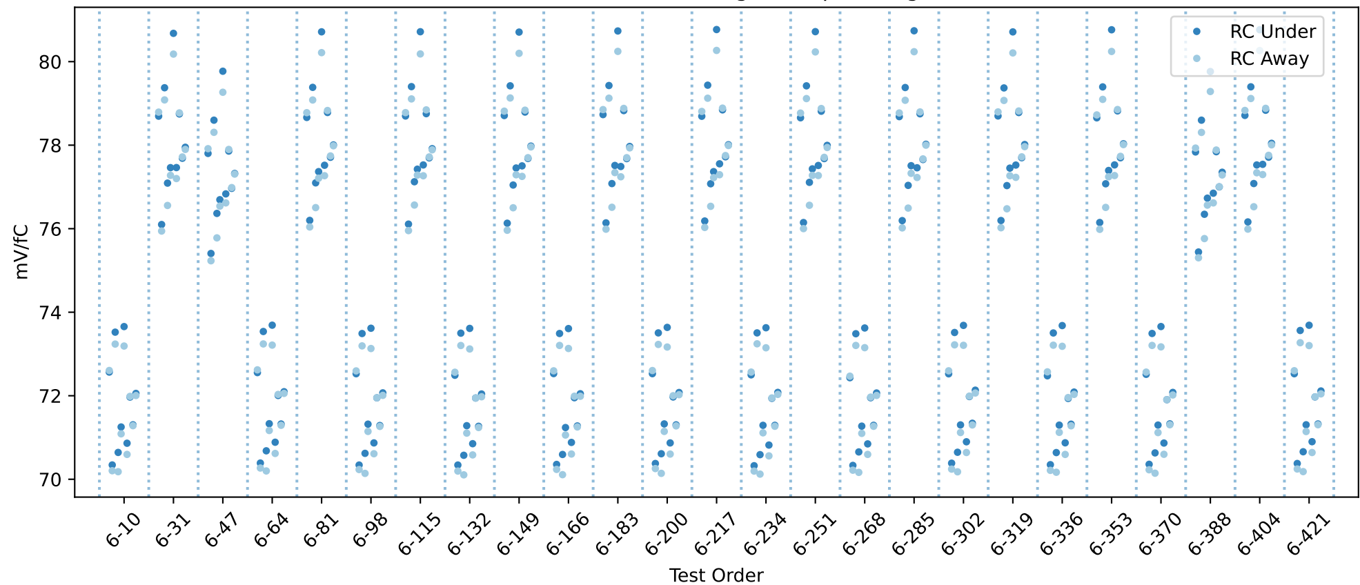
20USBHX2007938 RC gain chip averages
