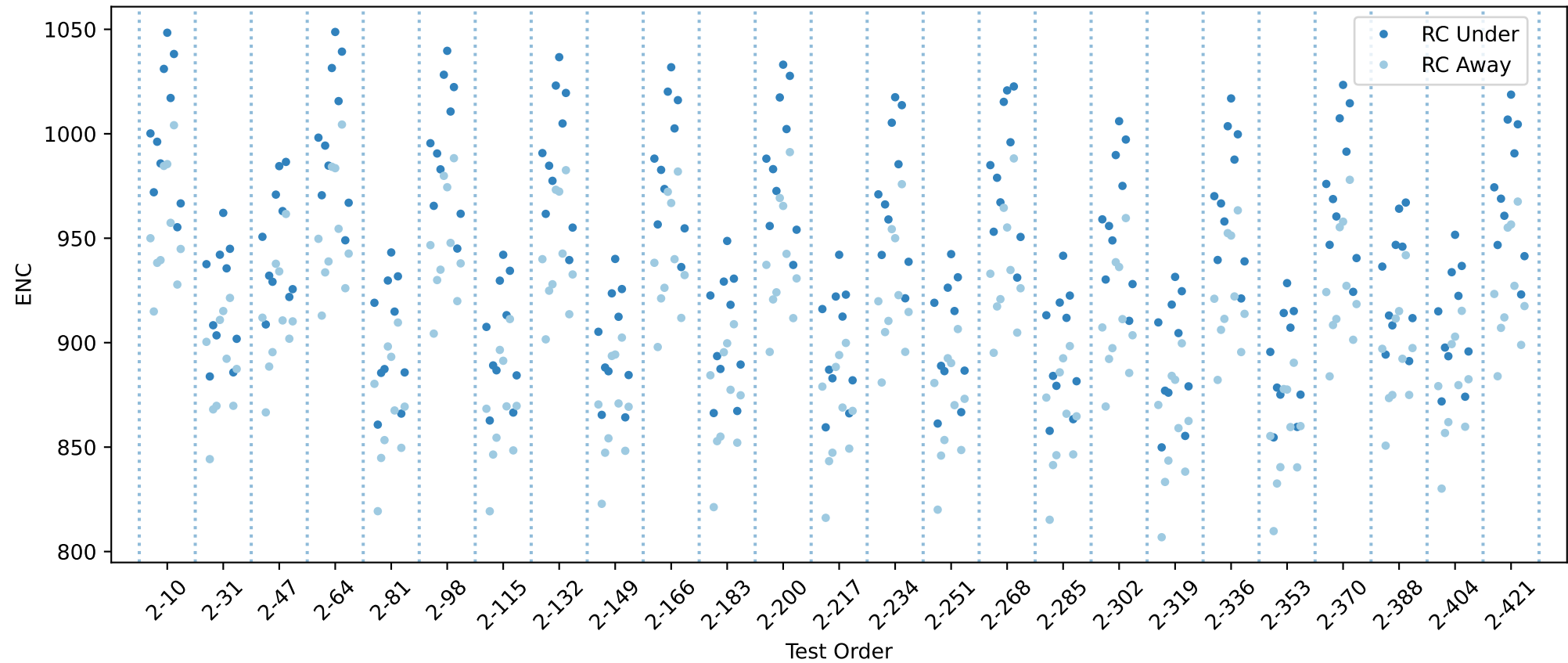
20USBHX2007925 RC innse chip averages
