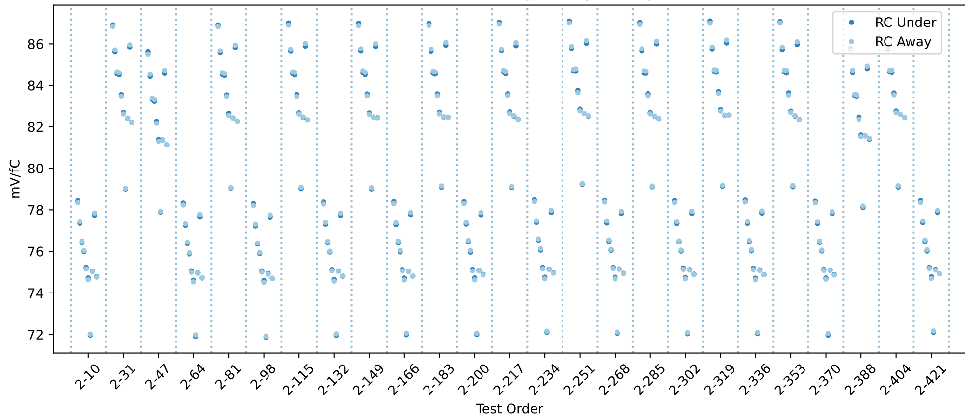
20USBHX2007927 RC gain chip averages
