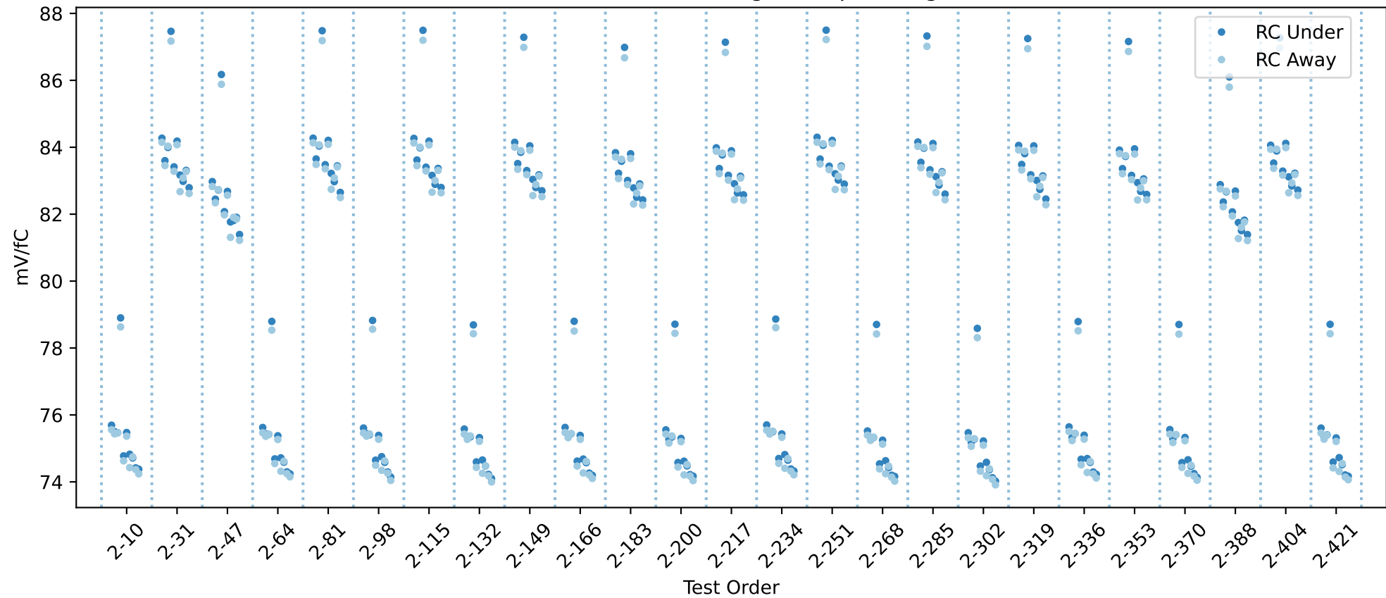
20USBHX2007929 RC gain chip averages
