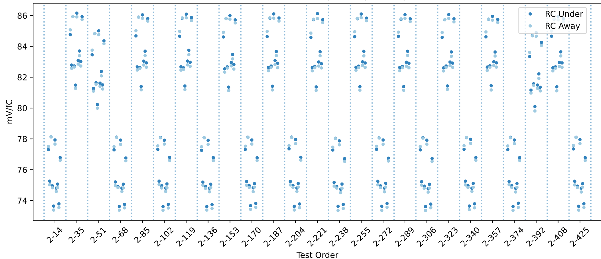
20USBHX2007922 RC gain chip averages
