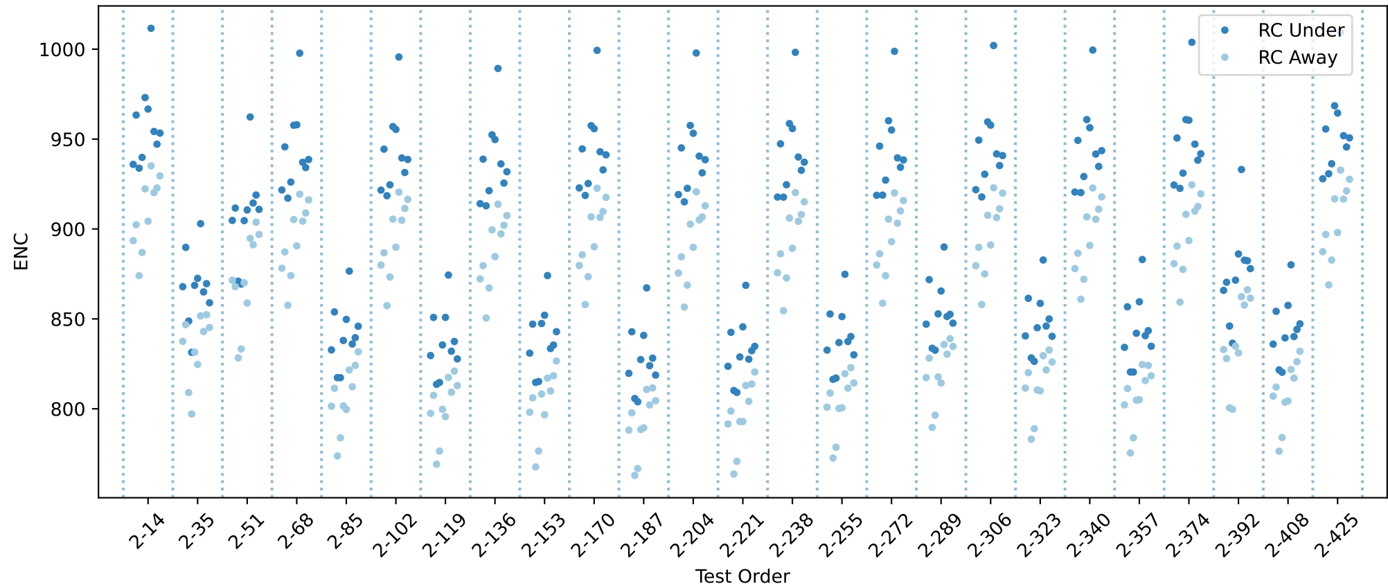
20USBHX2007935 RC innse chip averages
